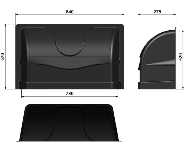
AeroHood 850
