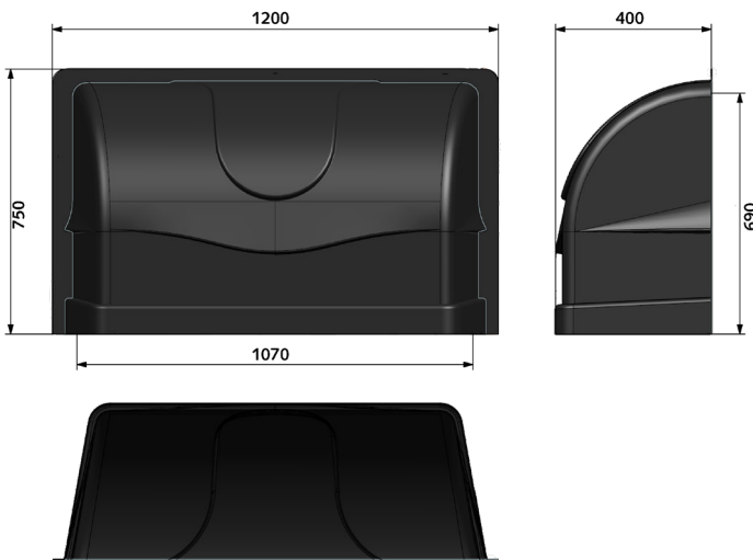
AeroHood 1200
